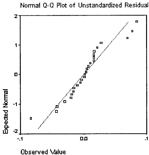
Gambar 4.1. Distribusi Normalitas Residu
